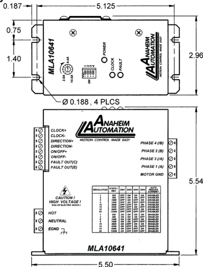
Figure 1: MLA10641 Dimensions
